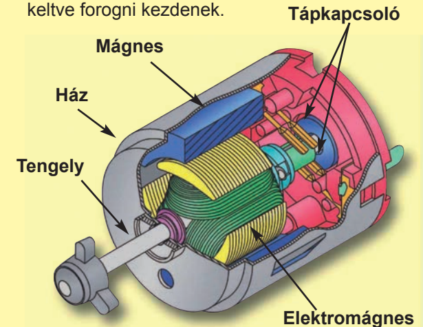
Motor (M1)
